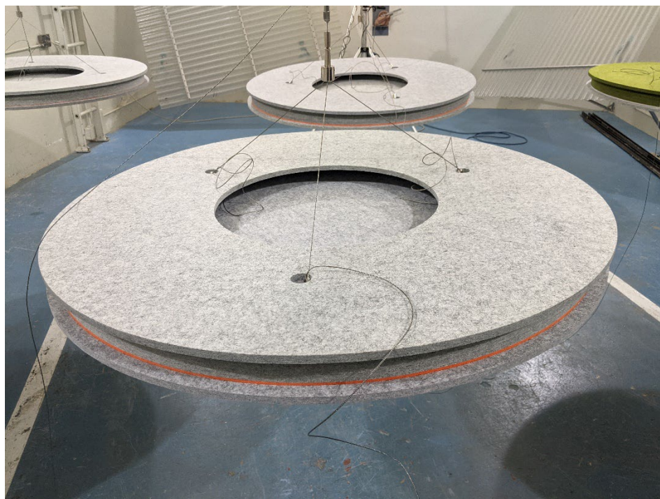
Figure 2 – Detail of individual baffle prior to installation of added felt strip
