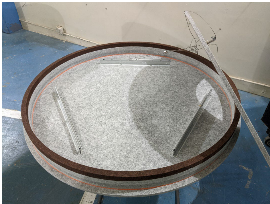
Figure 3 – Detail of added felt strip (brown felt ring) installed to individual baffle; baffle top temporarily removed
