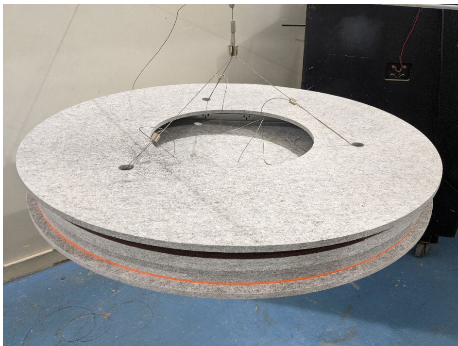
Figure 4 – Individual specimen baffle after installation of added felt strip
